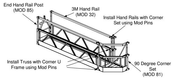
Install Hand Rail Post, Hand Rails and Install 90 Degree Corner Set
