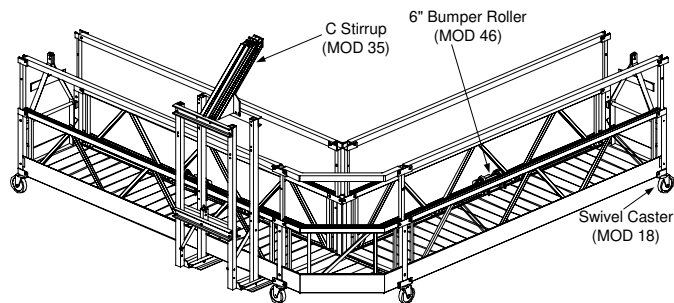
Install C Stirrup, Bumper Rollers and Swivel Casters
