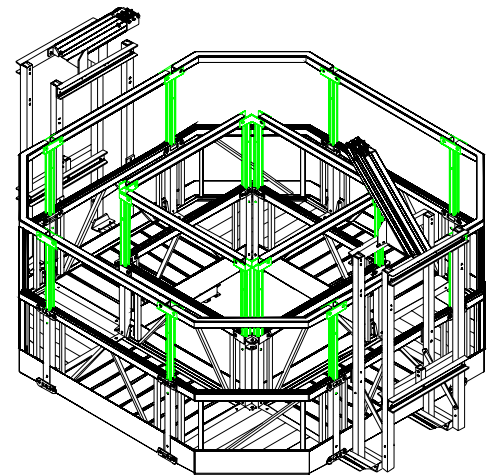
90 Degree Square or Rectangular Platform
