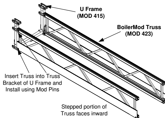
Install BoilerMod Truss with BoilerMod U Frame
