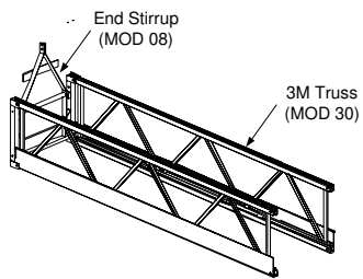
Install End Stirrup (MOD 08) with 3 M Trusses (MOD 30)
