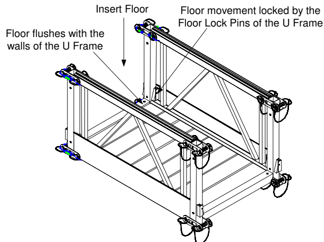
U Frame (MOD 05) with Floor Panel
