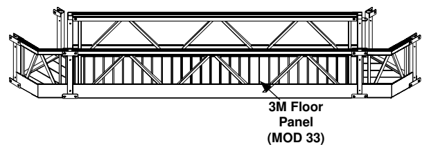
Install Floor Panels
