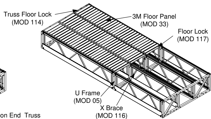
Install Floor Panels, Truss Floor Lock, Floor Locks and X Brace
