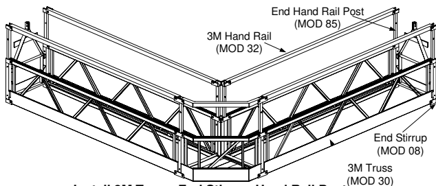
Install 3M Truss, End Stirrup, Hand Rail Post and Hand Rail with Corner Set
