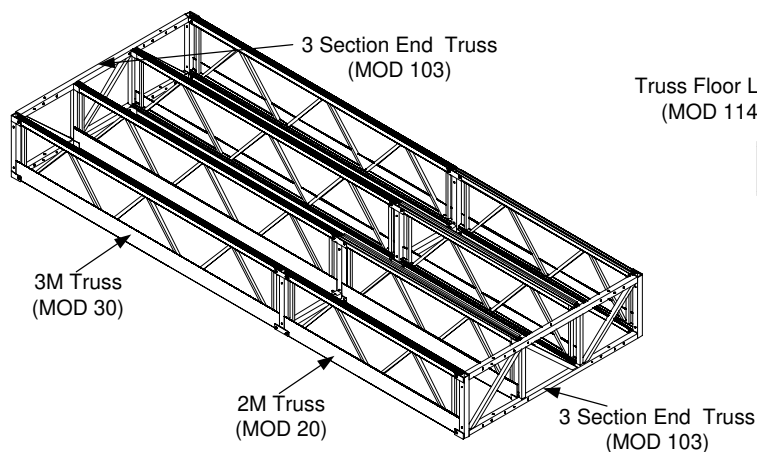
Base Frame of Super Deck
