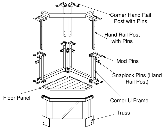
Corner Set Components
