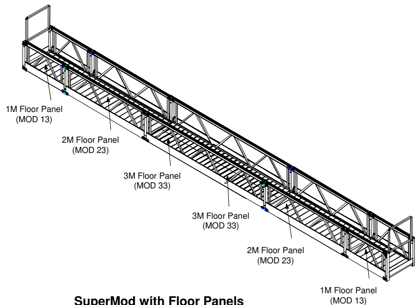
SuperMod with Floor Panels
