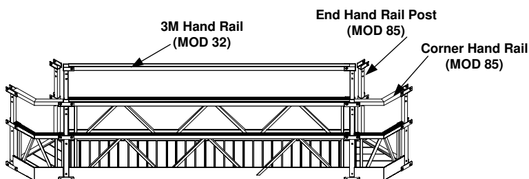
Install Hand Rail Posts and Hand Rails
