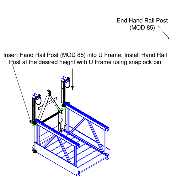
Hand Rail Post Installation
