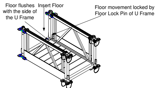
Floor Panel Installation
