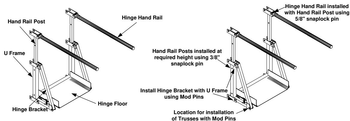
Hinge Set with U Frame and Hand Rail Posts
