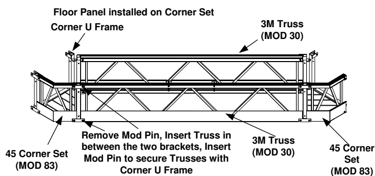
Install Trusses with Corner U Frames
