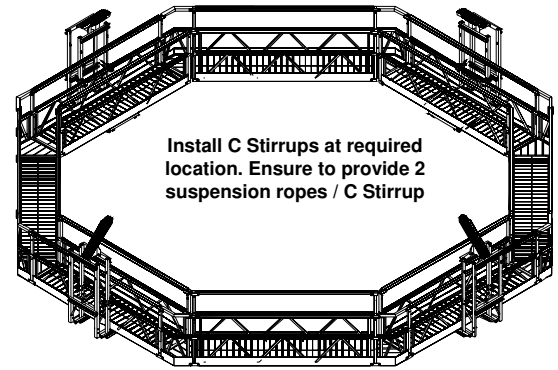
Circular Platform with C Stirrups
