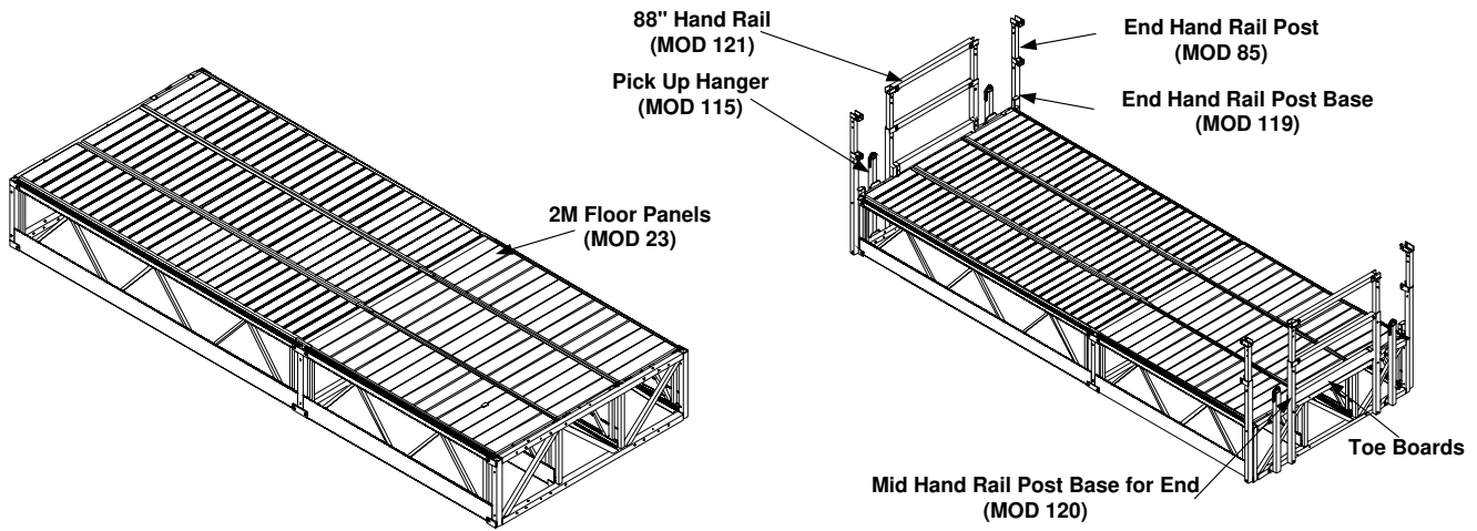
Super Deck with Floor Panels
