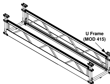
Install Subsequent U Frame with Trusses
