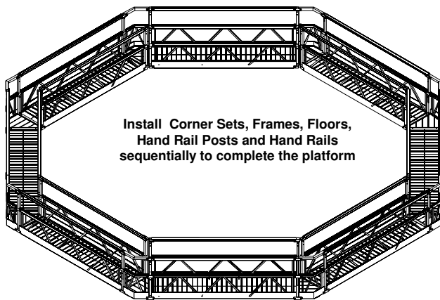
Framework of Circular Platform
