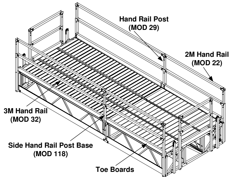
Super Deck with Floor Panels
