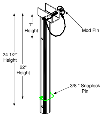
MOD 85: End or Inner Corner Hand Rail Post
