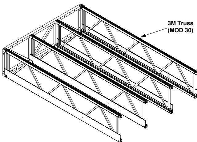
Install Trusses with End Truss
