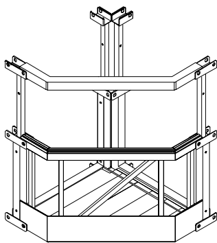
90 Degree Corner Set
